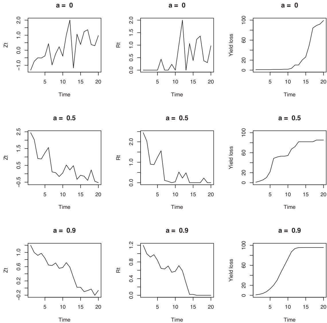
Fig. 1. Examples of the time series generated by the yield loss model. When \alpha=0 , the Z_t series is white noise. When \alpha=0.5 or \alpha=0.9 , the Z_t series is lighter pink and darker pink noise. As \alpha increases, the greater level of temporal autocorrelation produces a smoother series Z_t . In the no-yield-recovery model, the R_t series of 'weather conduciveness to yield loss from pests or diseases' (from Eq. (1)) has 0 as a minimum value. The resulting cumulative yield loss series (from Eq. (2)) also tend to be smoother for higher \alpha . The examples shown here are for m=0 and \sigma^2=1 in the no-yield-recovery model.
